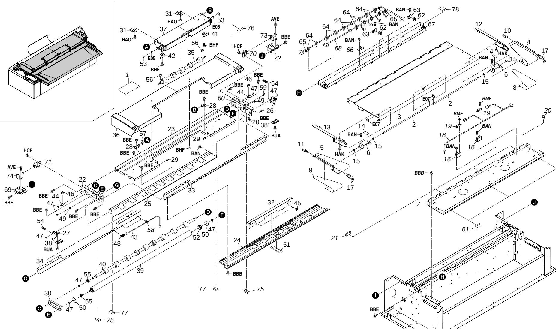
FIG. 3 ORIGINAL SET SECTION
