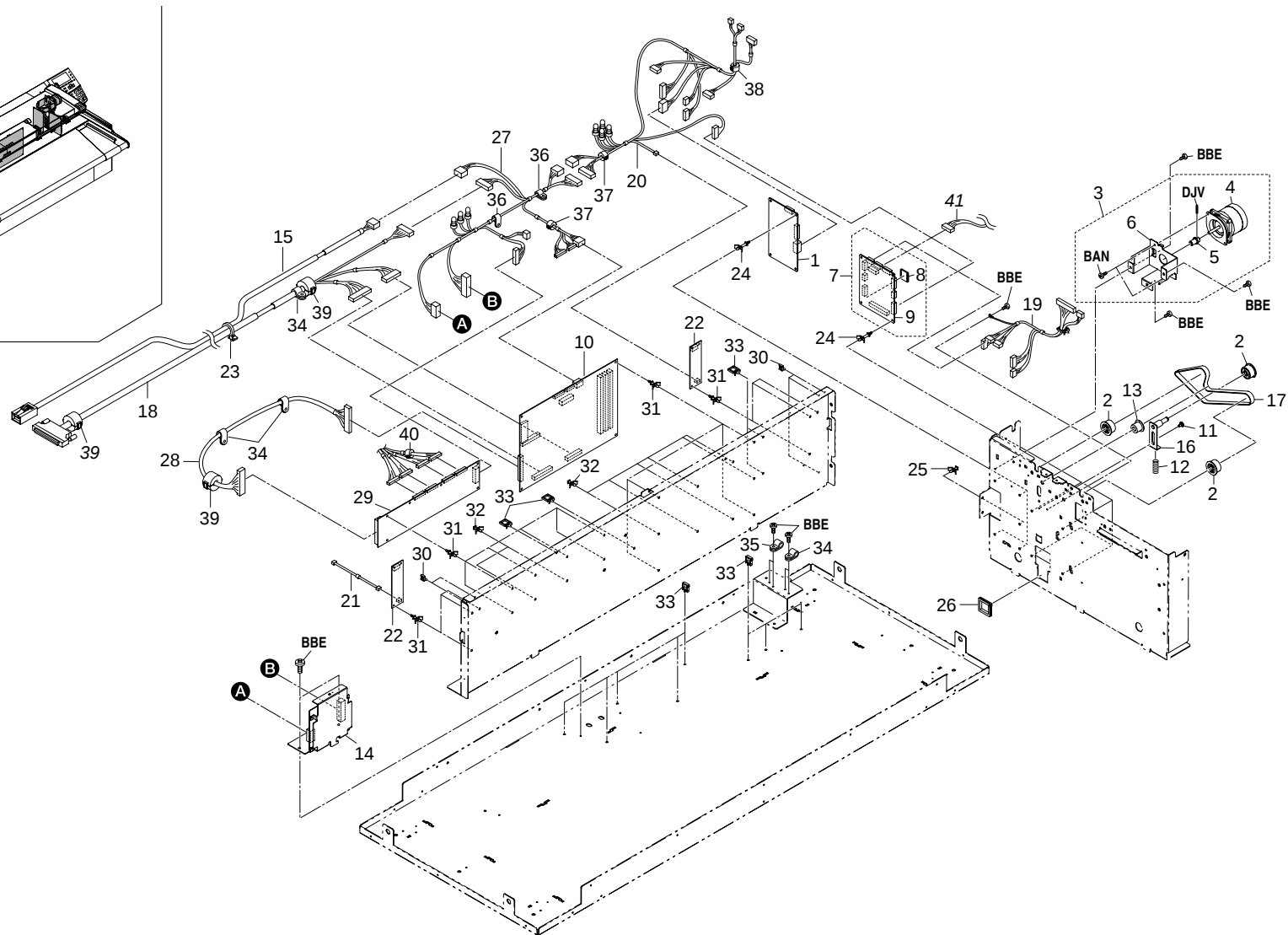
FIG. 4 DRIVING & ELECTRICAL COMPONENTS
